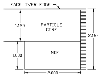
Birch Plywood Dropped Edge | WE09
